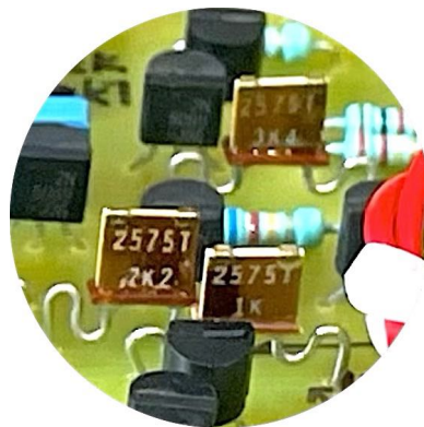
Texas Components TX2575 naked Z-Foil resistors
